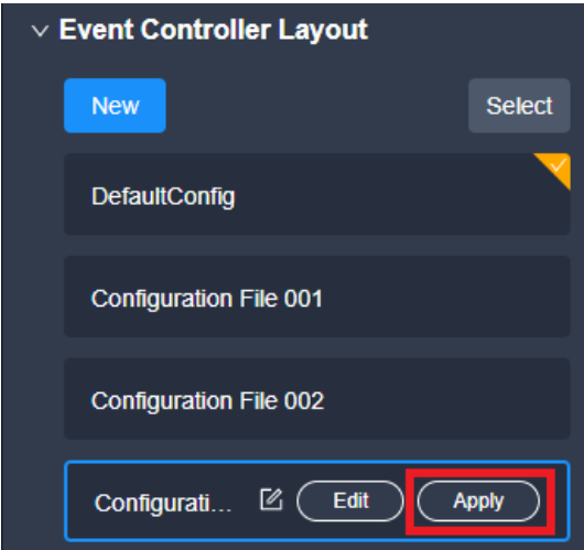
Figure 8-28 Applying
