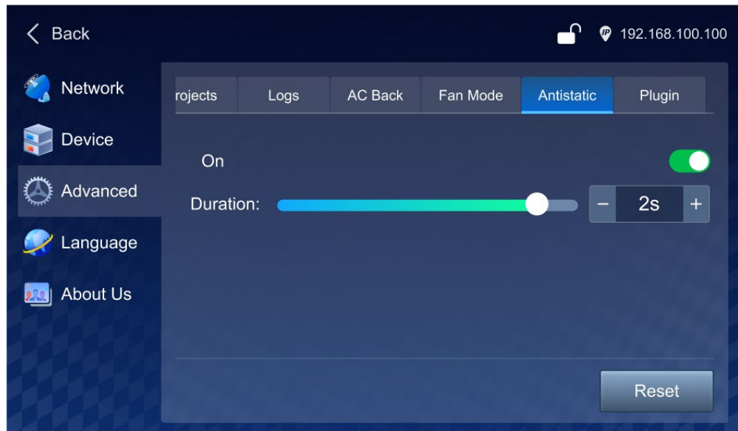
Figure 6-60 Antistatic settings
