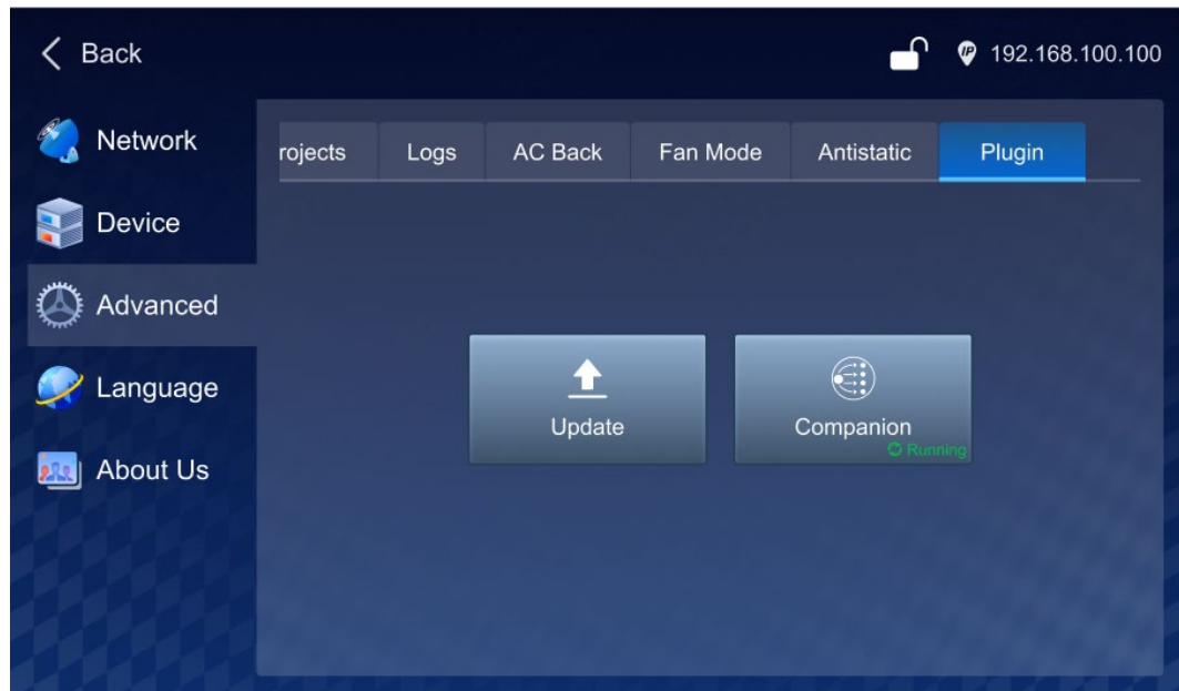
Figure 6-61 Plugin
