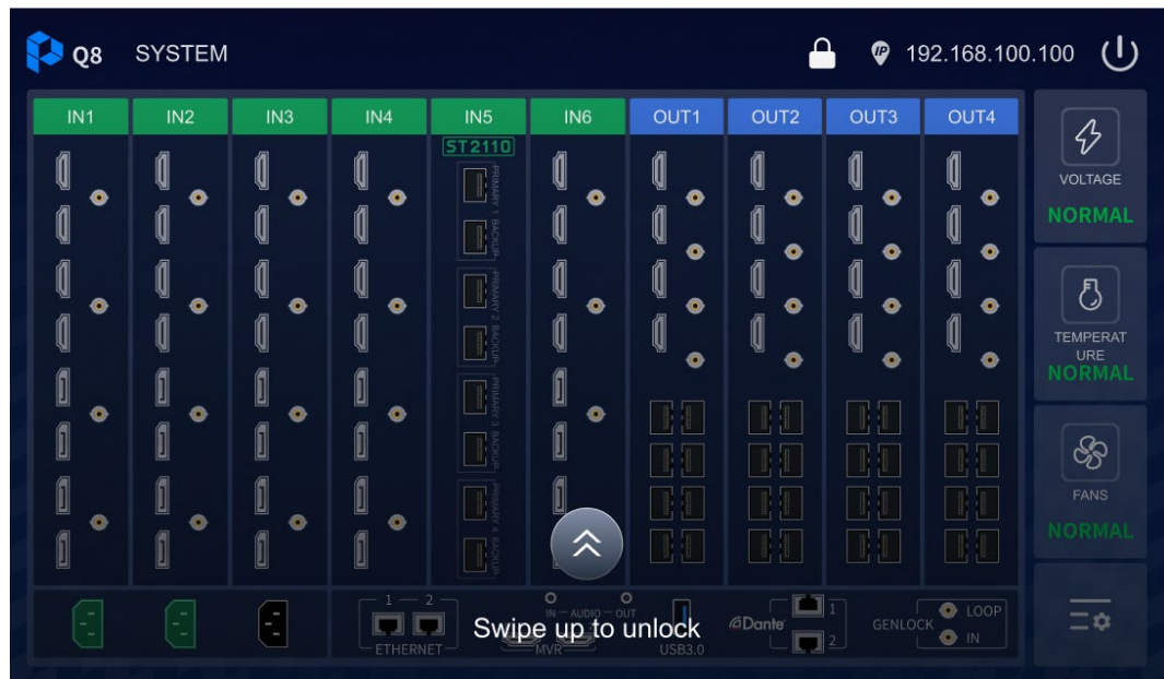
Figure 6-65 Unlock
