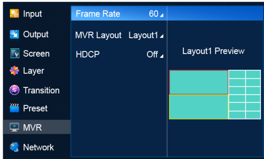
Figure 6-33 Multiviewer (P20)
