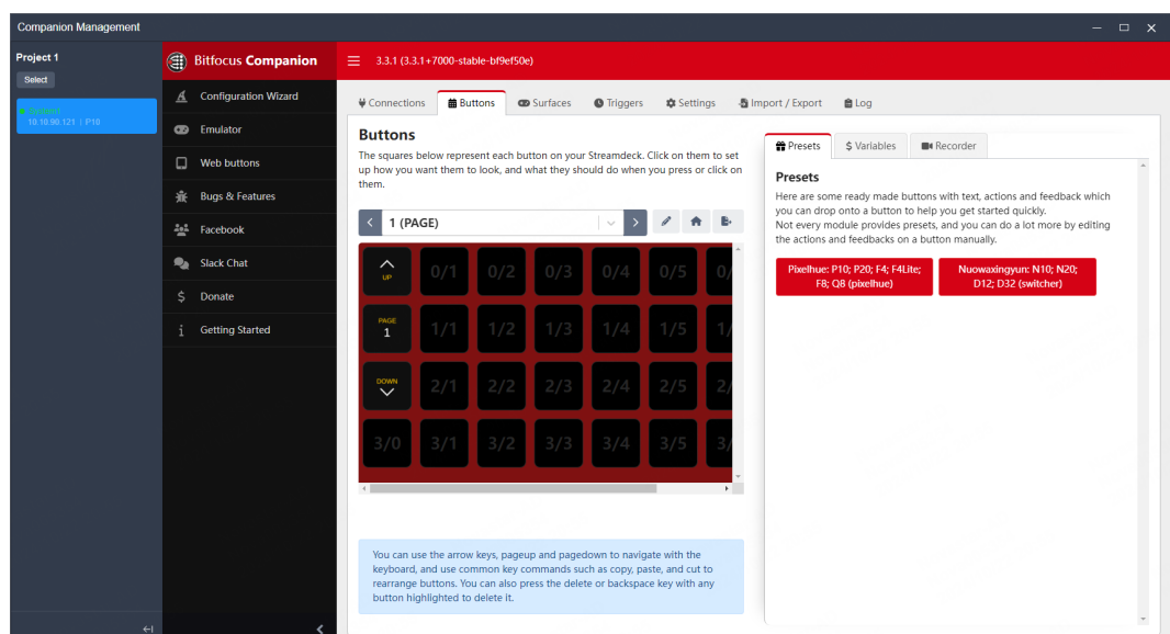
Figure 7-32 Button configuration
