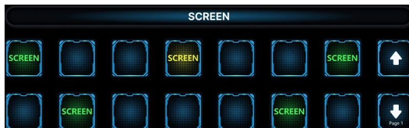
Figure 8-6 Screen buttons
