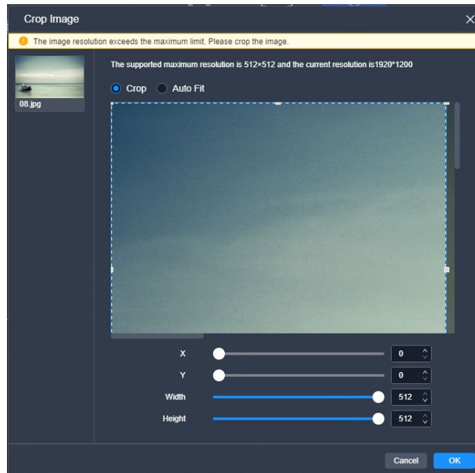
Figure 7-18 Crop images
