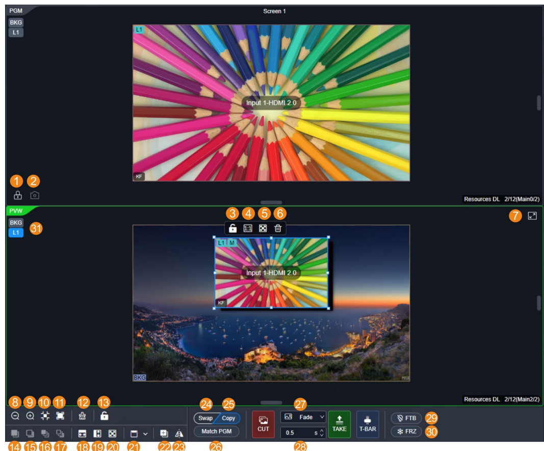
Figure 7-17 Layer operations
