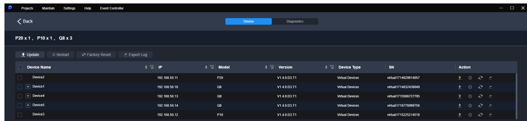
Figure 7-22 Device maintenance
