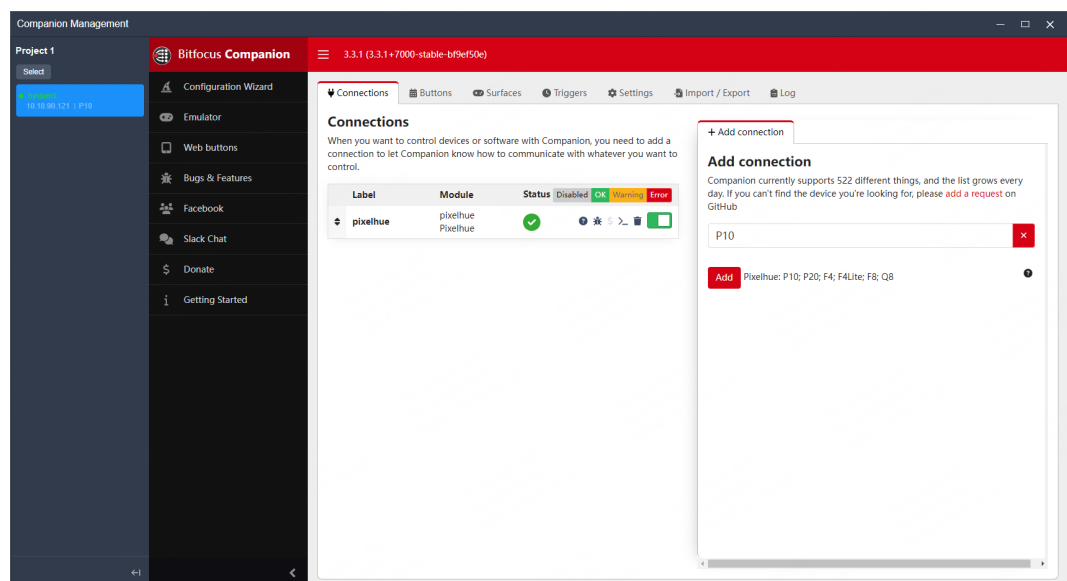
Figure 7-29 Search devices
