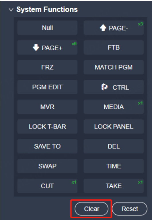
Figure 8-27 Clearing
