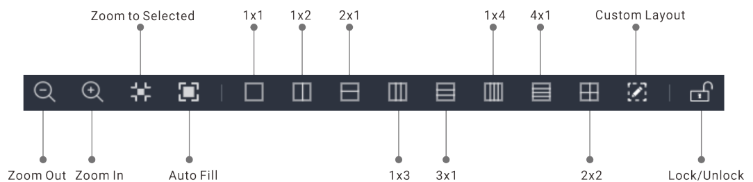
Figure 7-15 Toolbar (P20)
