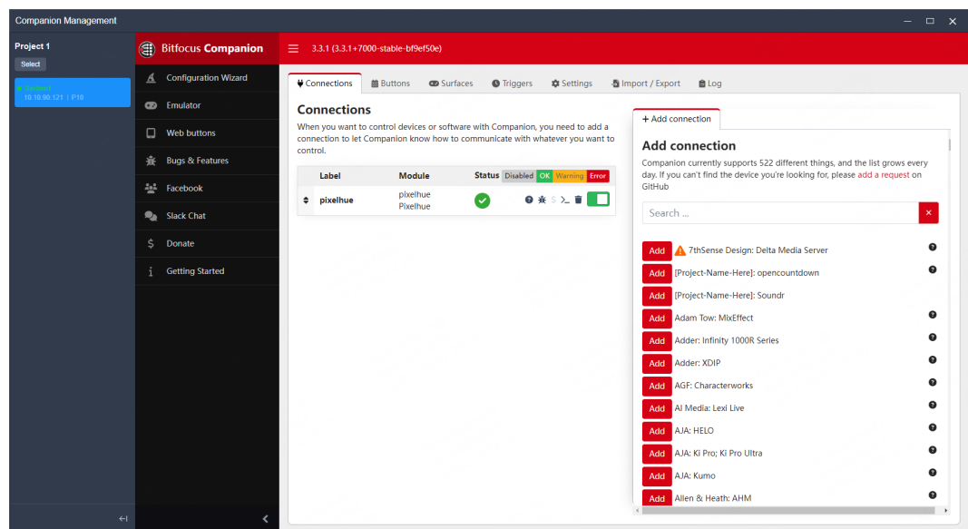
Figure 7-28 Companion management
