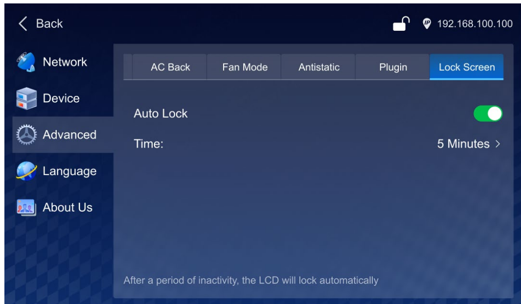
Figure 6-63 Lock screen
