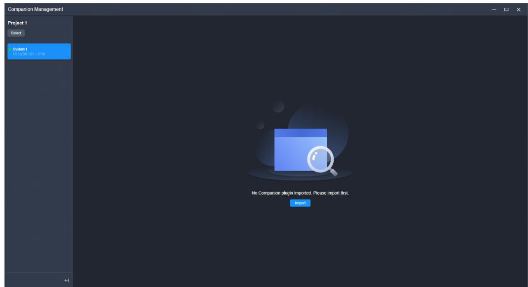
Figure 7-26 Companion management
