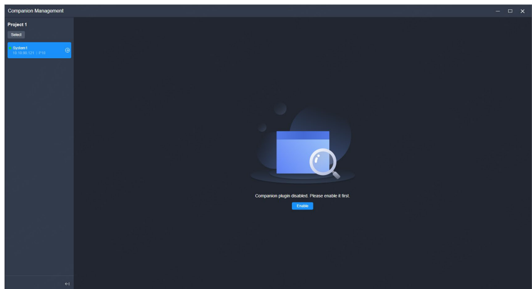
Figure 7-27 Enable plugin
