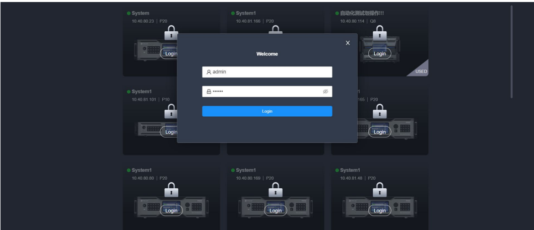
Figure 7-8 Device login
