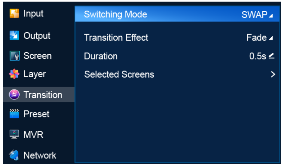
Figure 6-31 Switching (P20)
