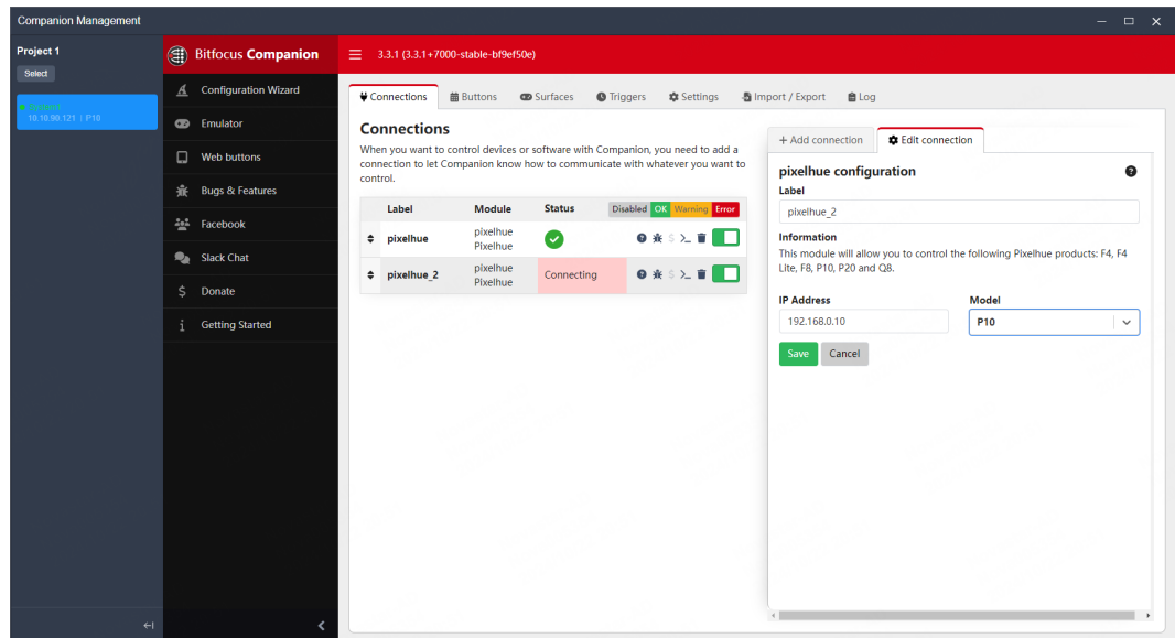
Figure 7-30 Edit connection
